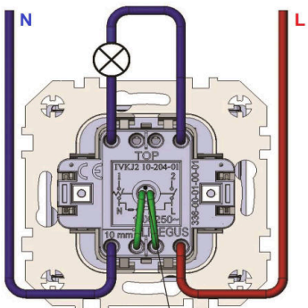
Illumination lamp(LED)
